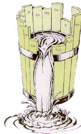
• Figure 6 - Law of Limiting Factors
