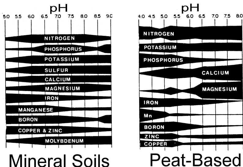
• Figure 2 - The Effect of pH on Nutrient Availability
