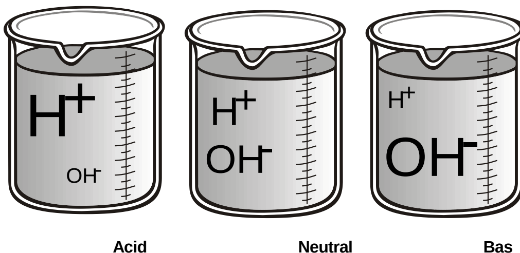
• Figure 1 - Relative Balance of Hydrogen/Hydroxide Ions
