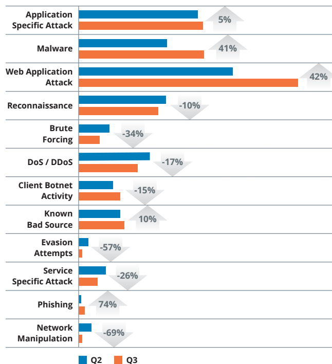
Figure 3: This graph represents the attack volume differences for attack categories across all industries between Q2 '17 and Q3 '17.
